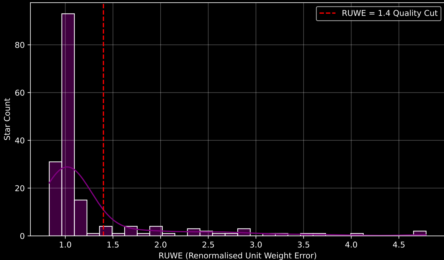
GAPOGEE DR17 Field [100+60] RUWE Distribution (n= 172)
