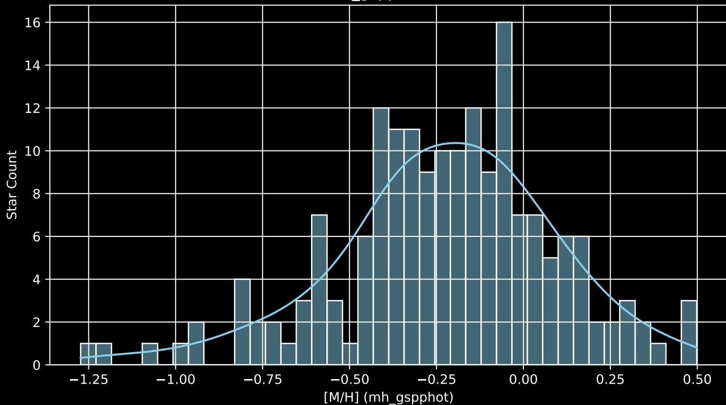
APOGEE DR17 Field: [100+60 [M/H] (mh_gspphot) (n= 179)
