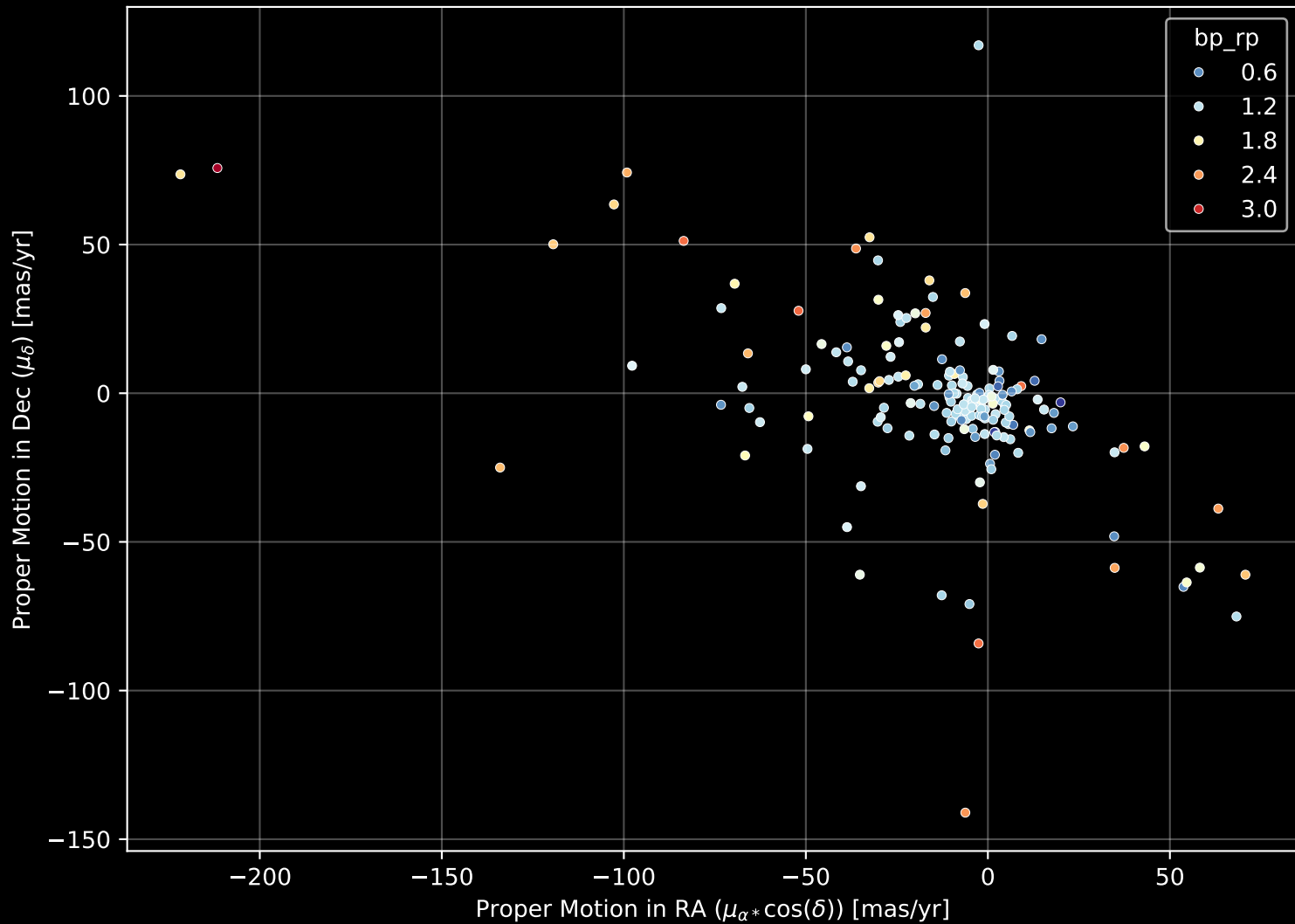
APOGEE DR17 Field: [100+60] Proper Motion Diagram (n= 181)
