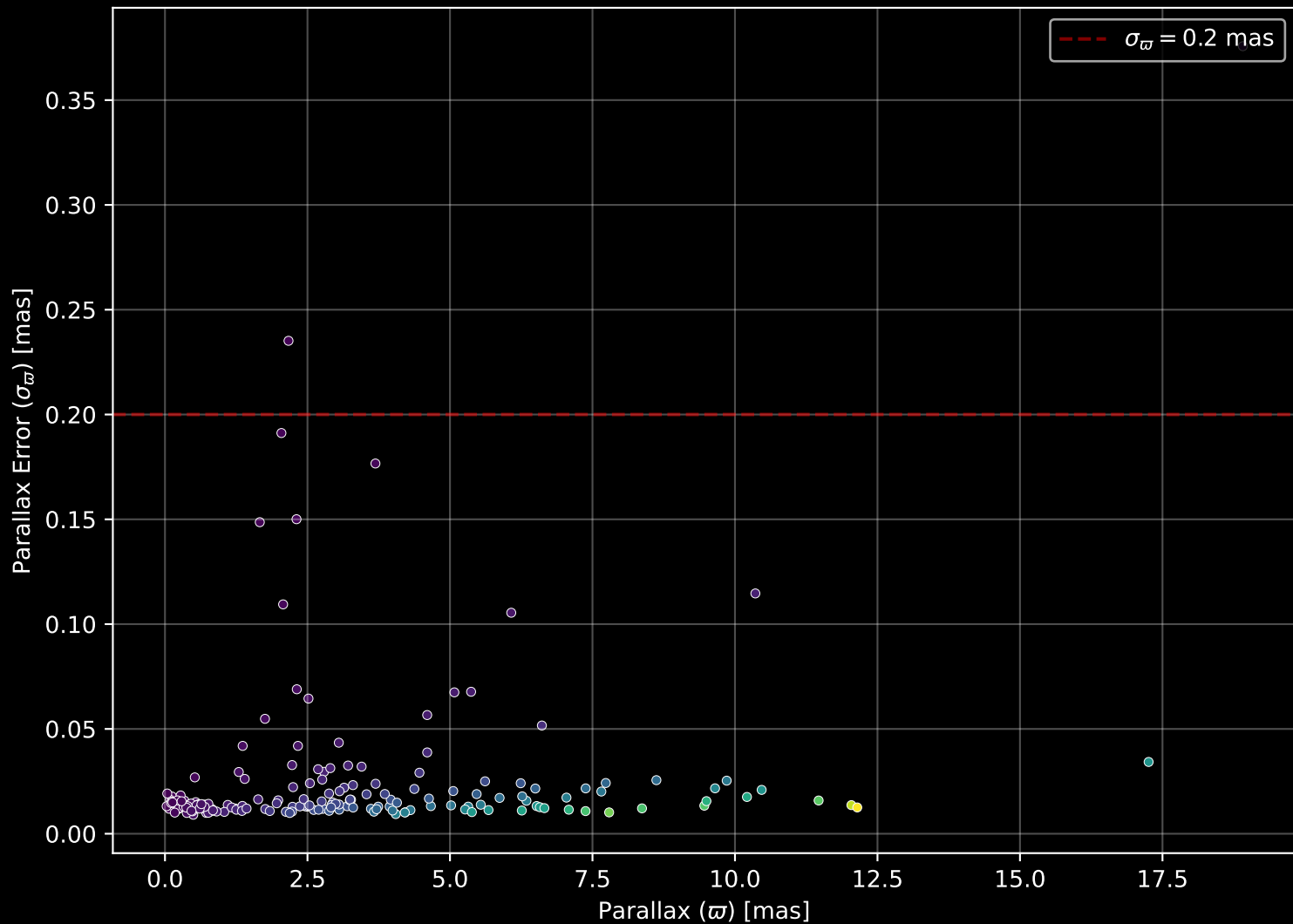
APOGEE DR17 Field: [100+60] Parallax Quality (n= 181)
