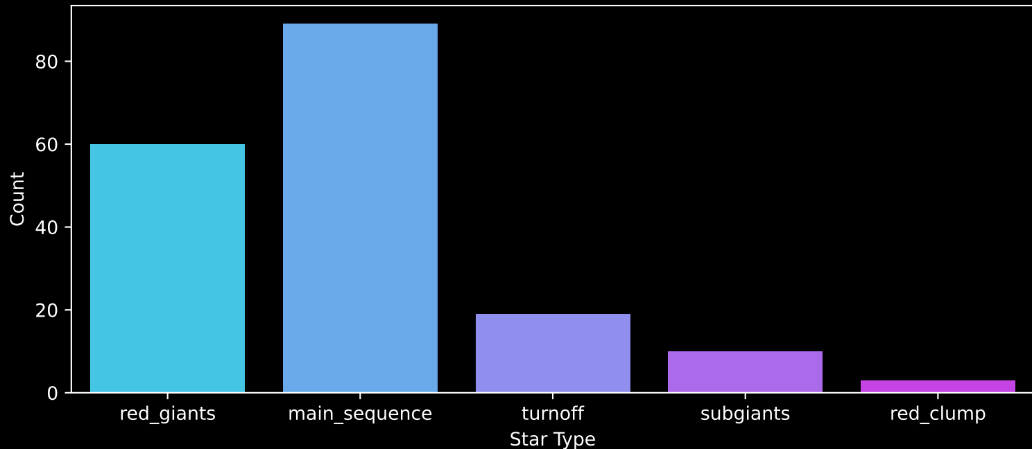
APOGEE DR17 Field: [100+60] Count plot of Star Type
